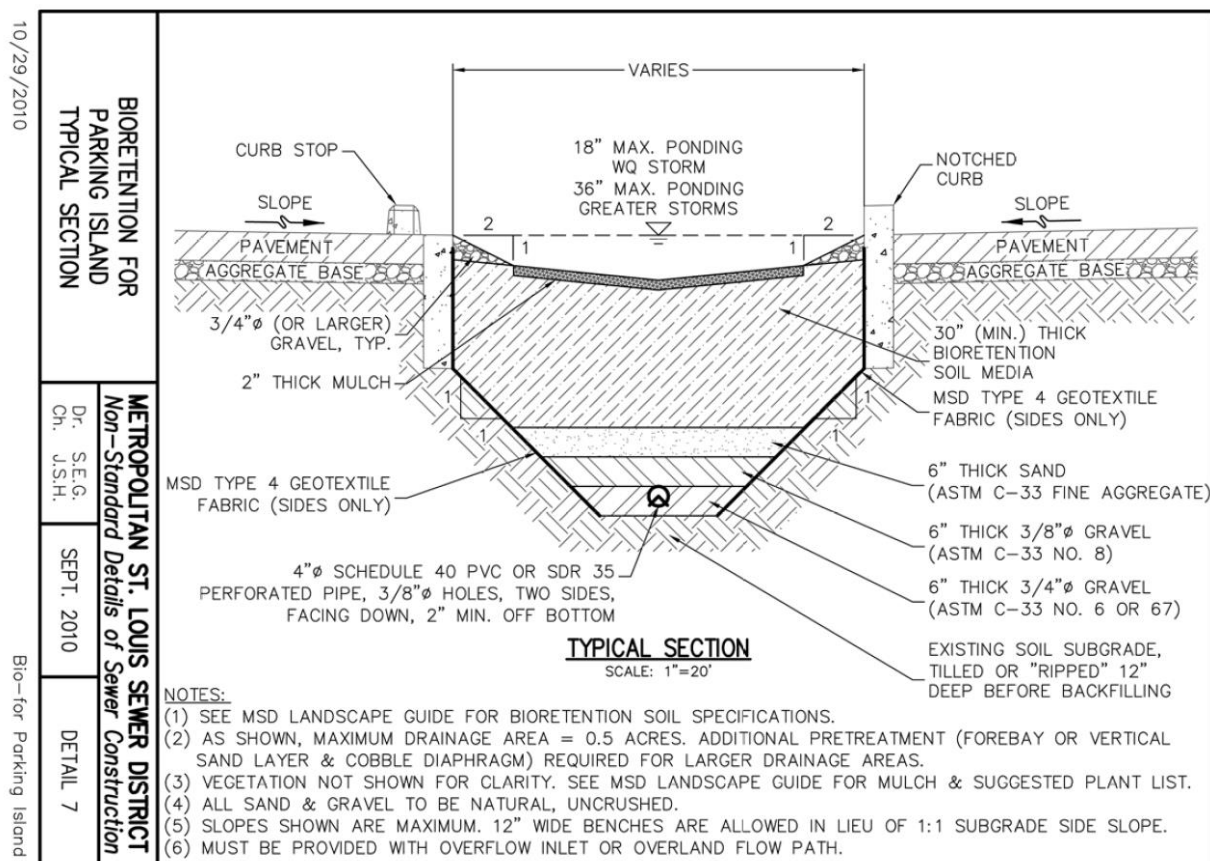
Fig 11. Metropolitan St. Louis Sewer District Bioretention Detail 1
