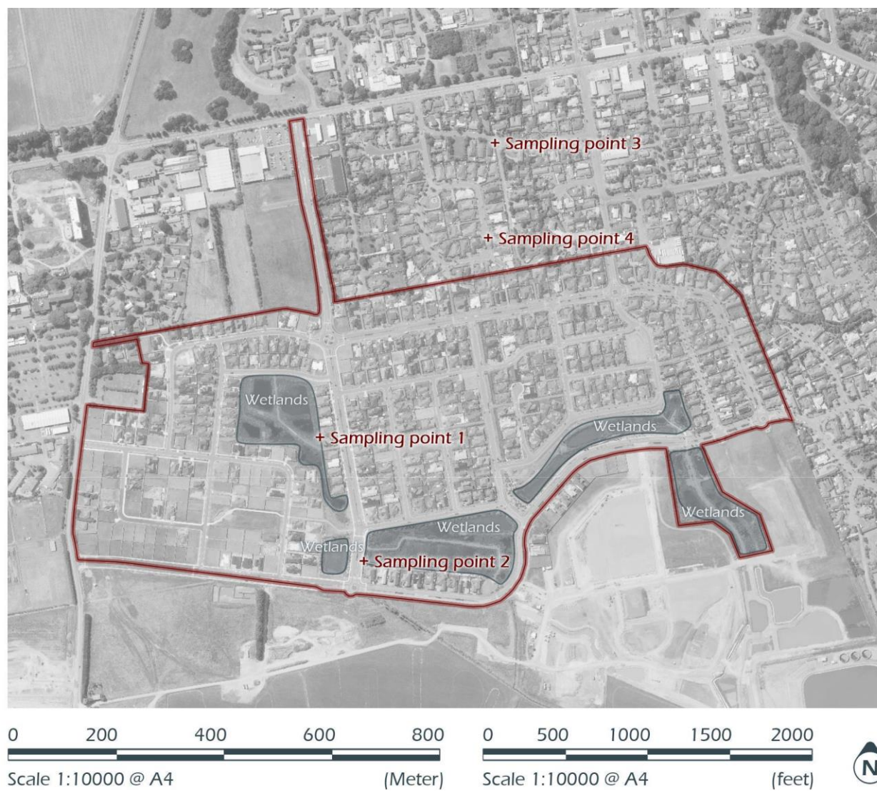
Figure 4. Four locations were sampled to represent the wetland-front residential areas and conventional areas
